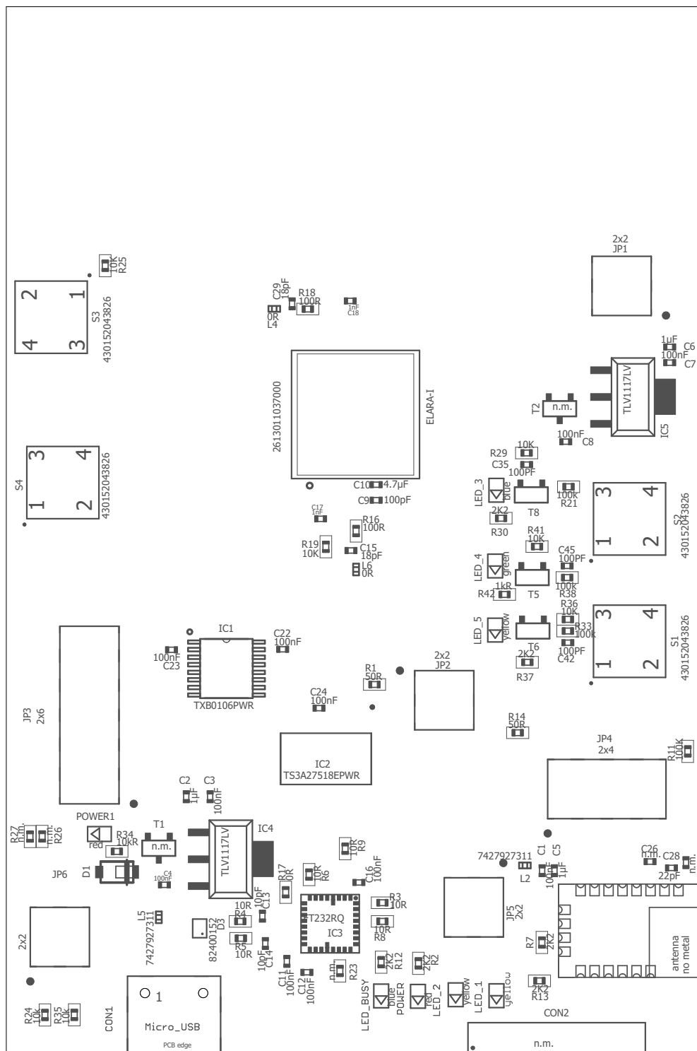
Figure 10: Assembly diagram
