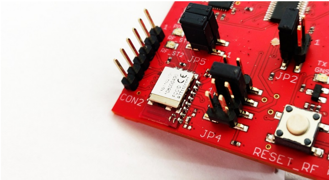
Figure 2: 2613019037011 - detail of the Thyone-I RF interface
